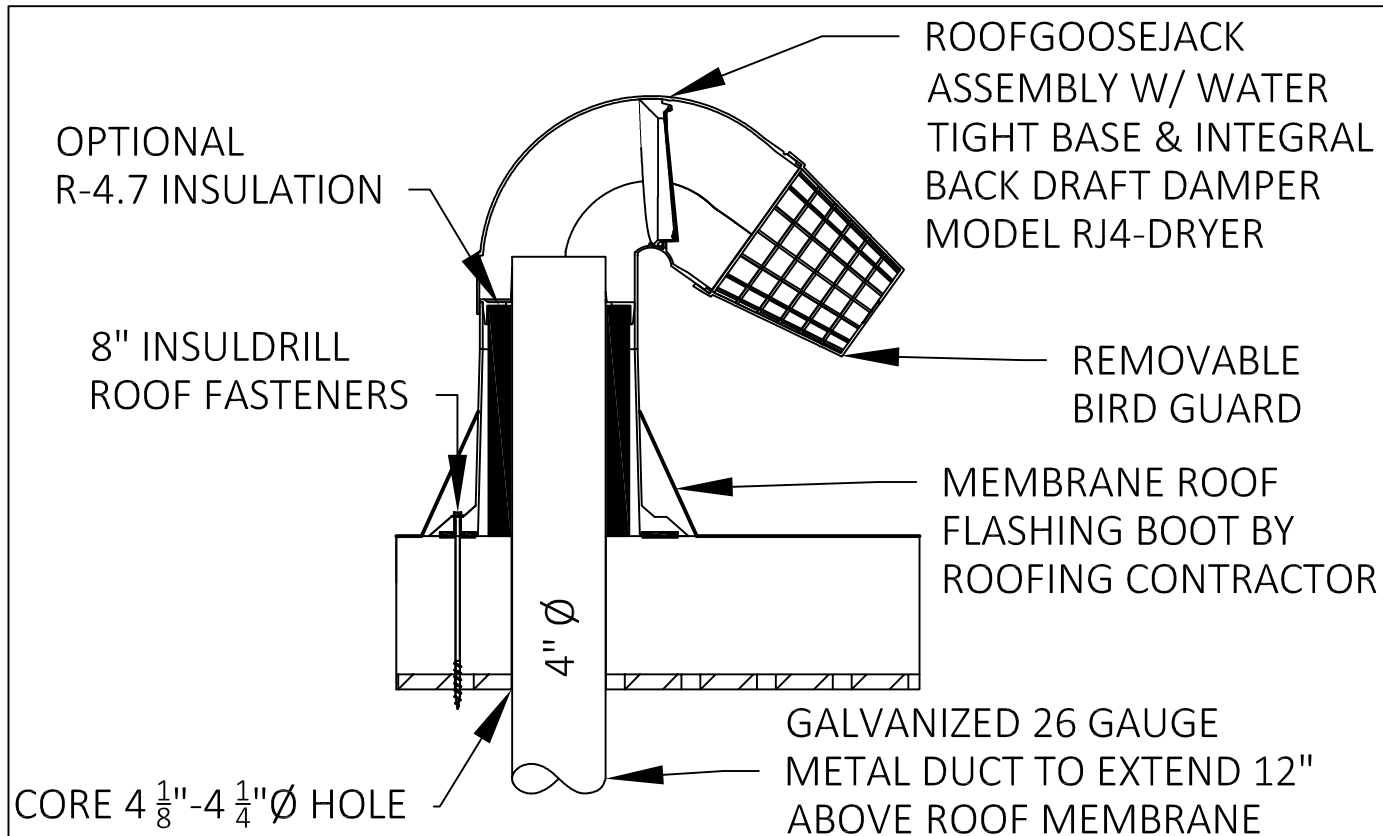
④ RJ4-IE TERMINATION INSTALL DETAIL NOT TO SCALE
