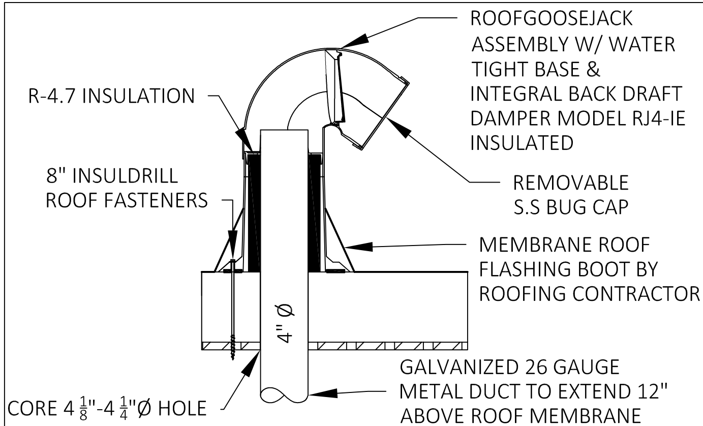
⑥ RJ4-IE INSULATED TERMINATION INSTALL DETAIL NOT TO SCALE
