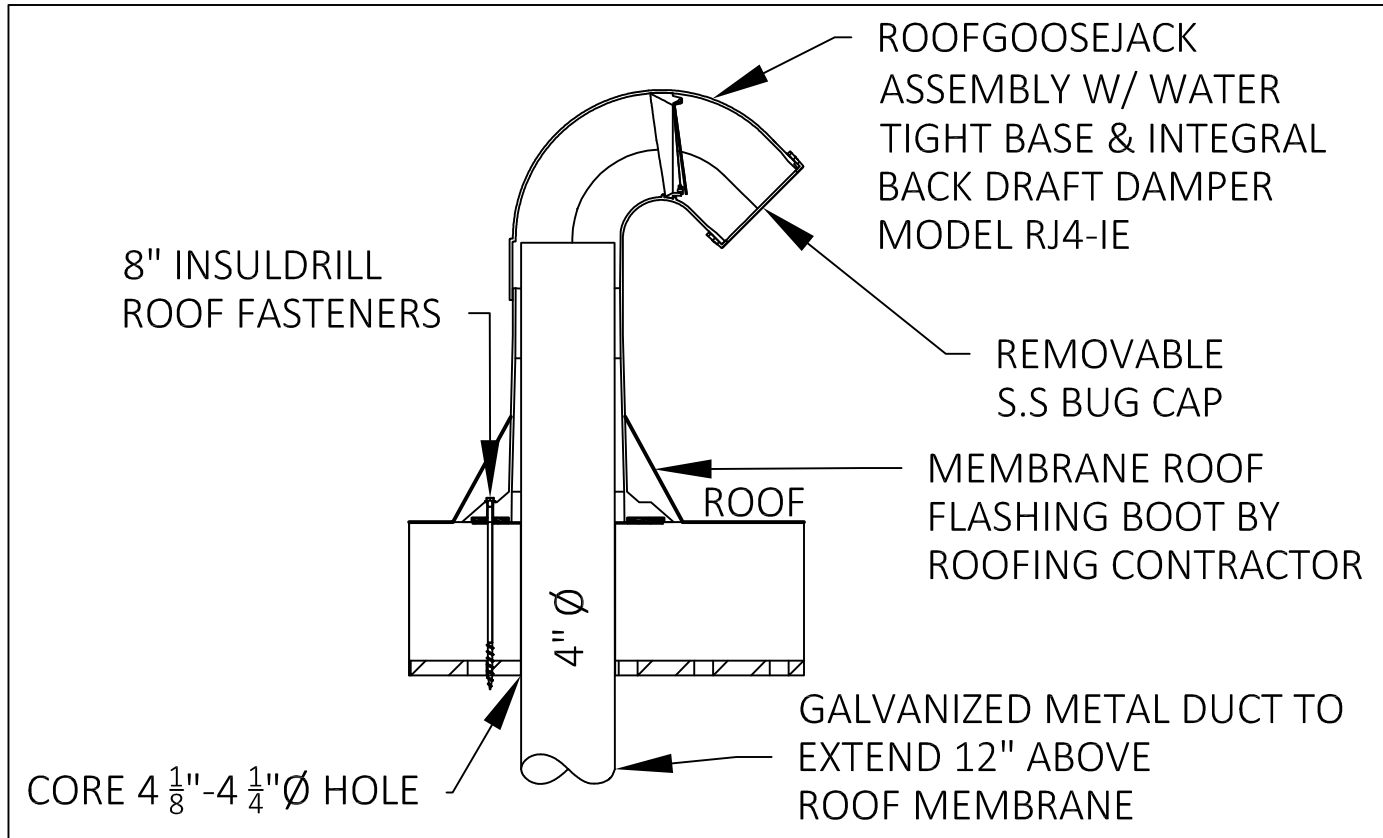
③ RJ4-IE TERMINATION INSTALL DETAIL NOT TO SCALE
