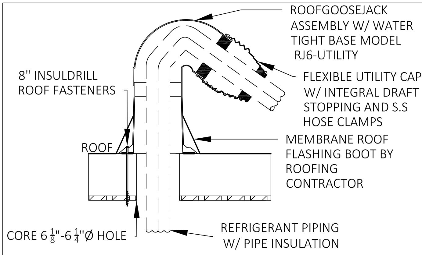
② RJ6-UTILITY TERMINATION INSTALL DETAIL NOT TO SCALE
