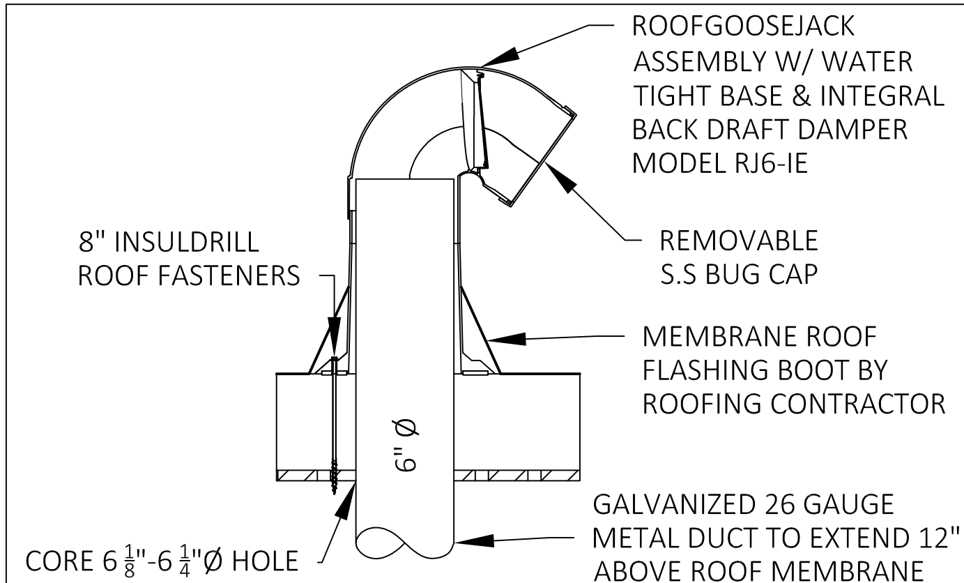
⑤ RJ6-IE TERMINATION INSTALL DETAIL NOT TO SCALE
