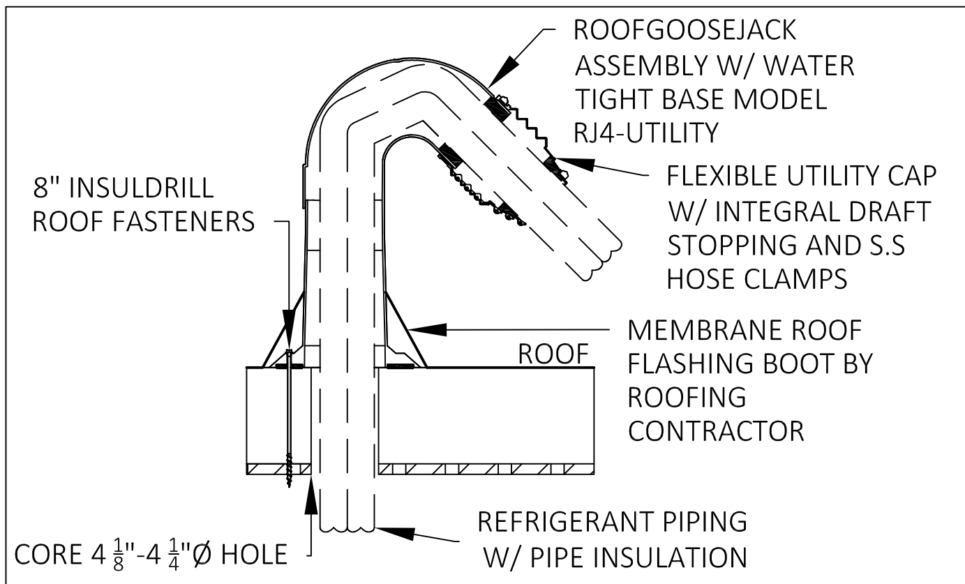
① RJ4-UTILITY TERMINATION INSTALL DETAIL NOT TO SCALE
